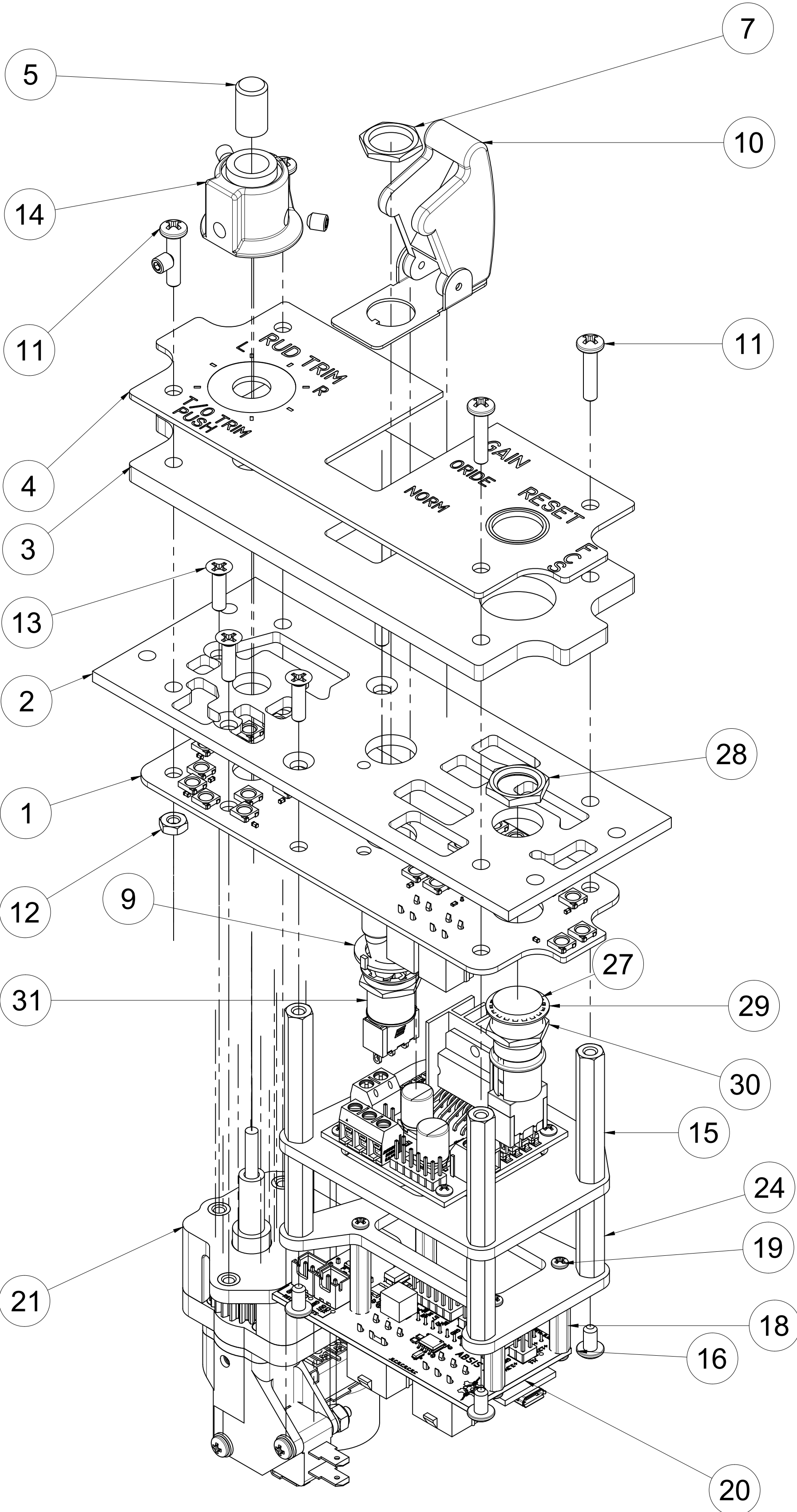
-1 ASSY SCALE 1.2:1
